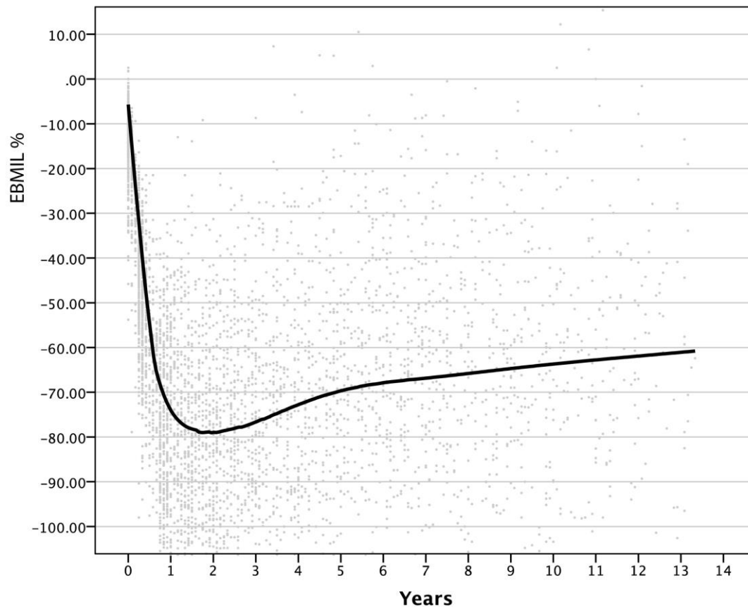
Figure 3a. Postoperative weight loss expressed as percentage of excess BMI loss (%EBMIL) plotted against time. The lines are drawn using locally weighted scatter plot smoothing method (lowess).
